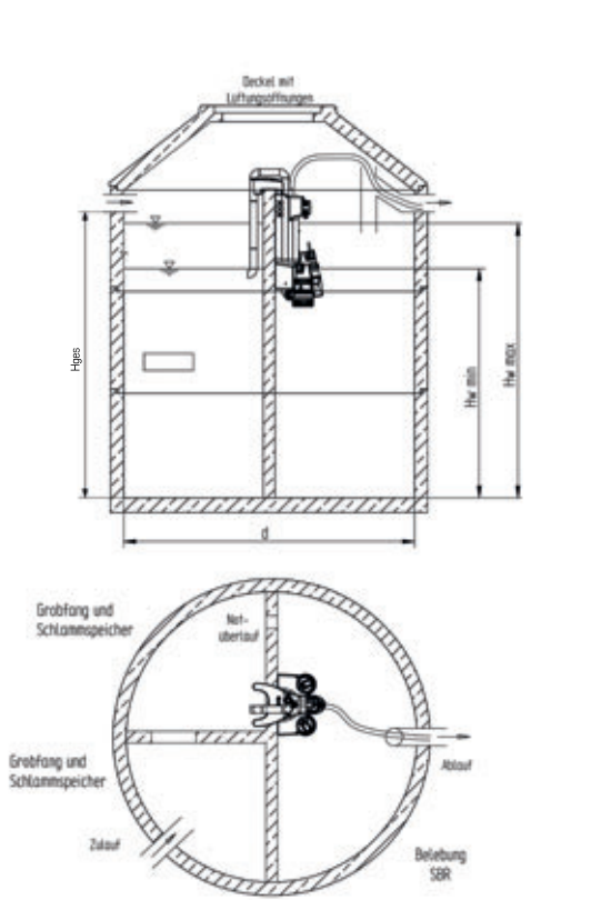
AQUAPRIMO® P Version M = Trennwandmontage
